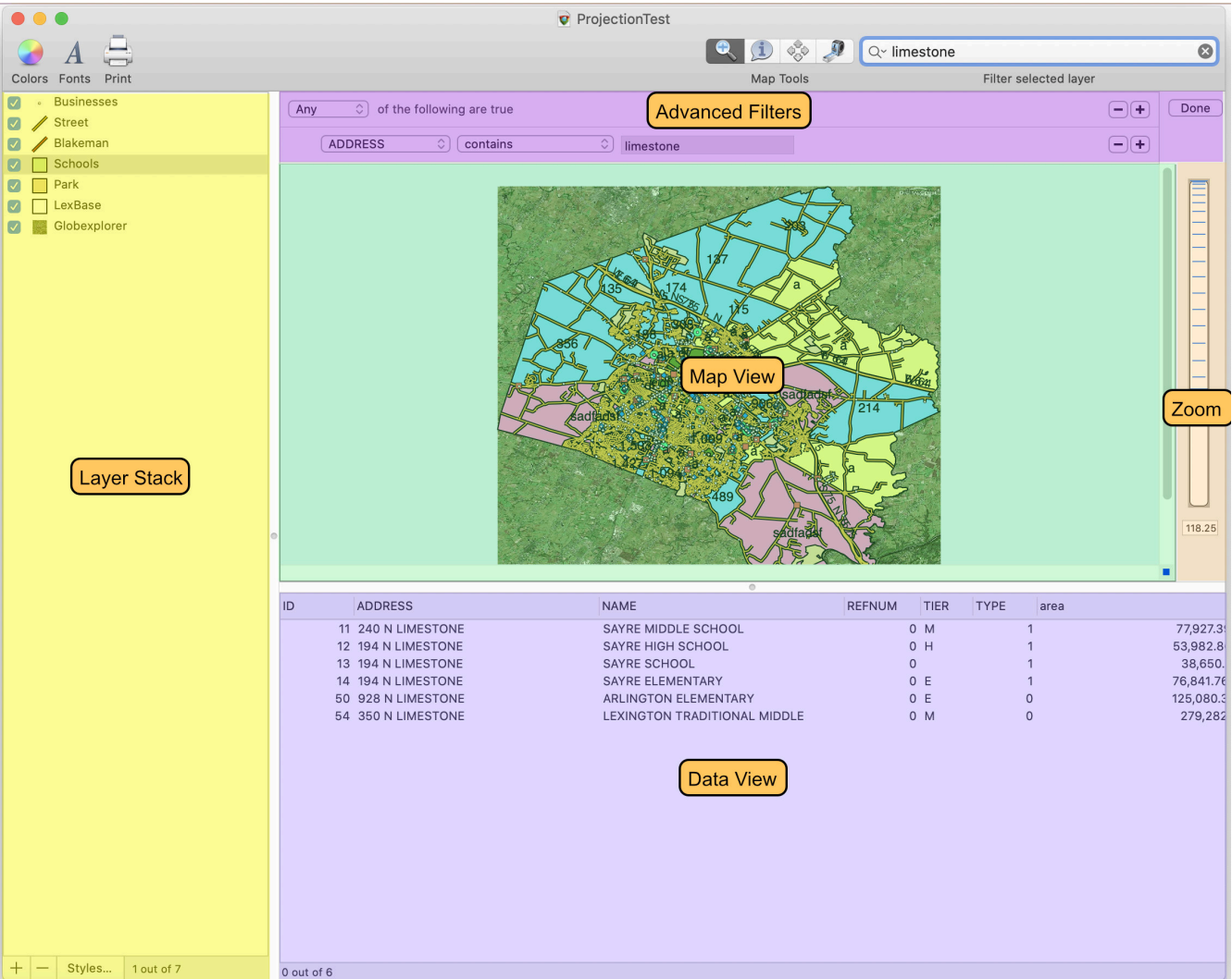
Main Cartographica Window
